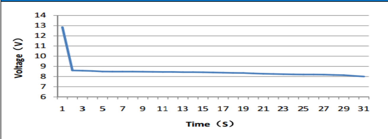
Cold Cranking Test Graph (-18°C, 850CCA)
